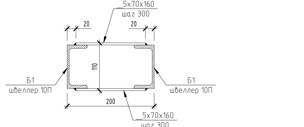
1-1 (M1:5)
